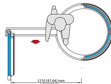
Large Controlled access transit Large Emergency egress Automatic sliding doors and swing door opening
