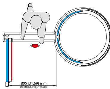
Emergency egress Manual swing door opening
