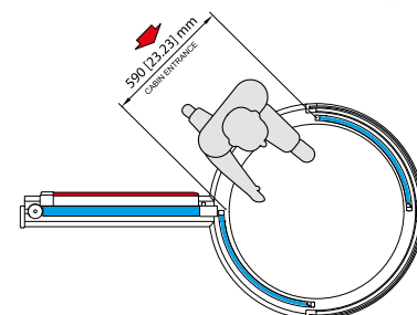
Controlled access transit Automatic sliding doors opening
